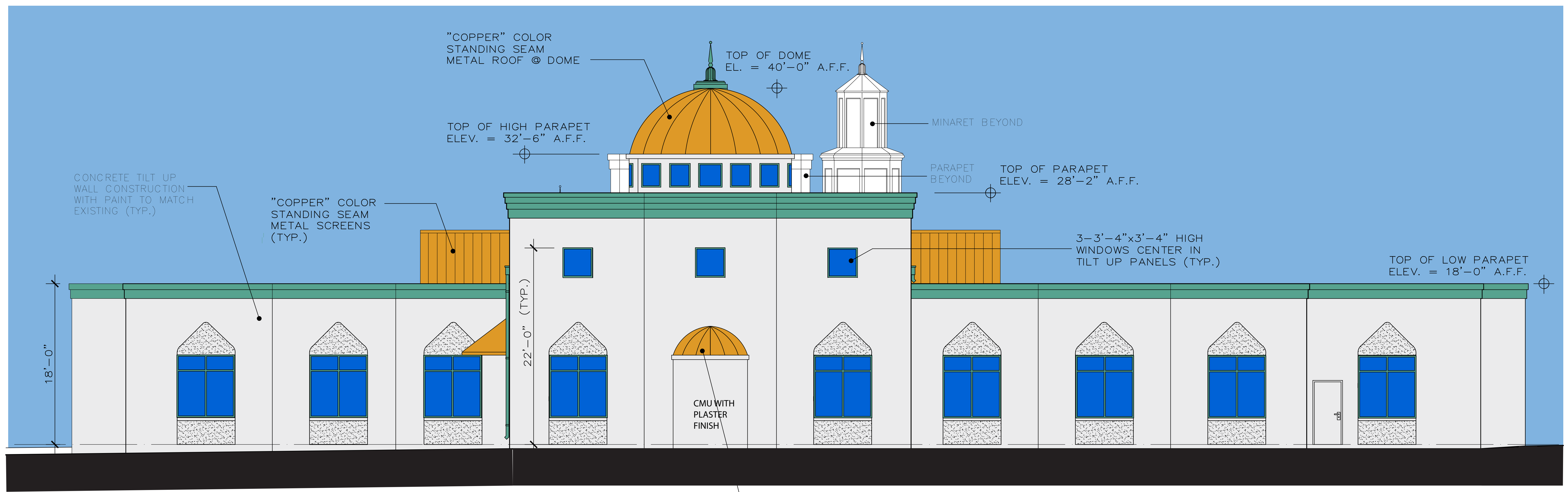
2 EAST / REAR EXTERIOR ELEVATION
