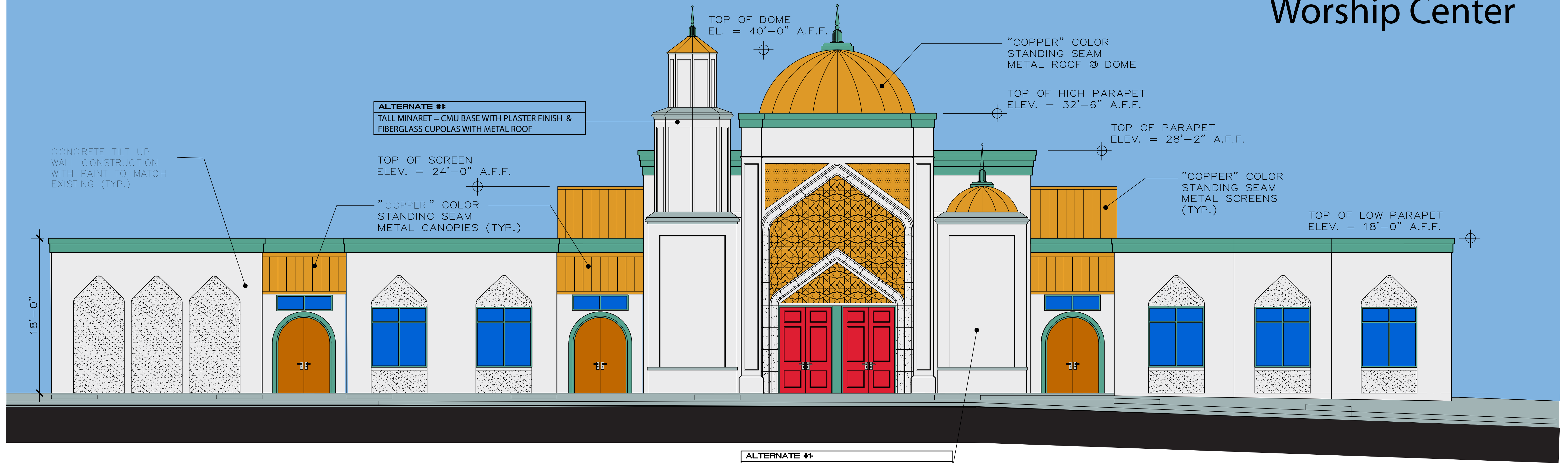
1 WEST / FRONT EXTERIOR ELEVATION
